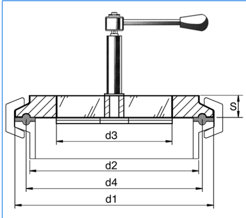
Typical assembly
