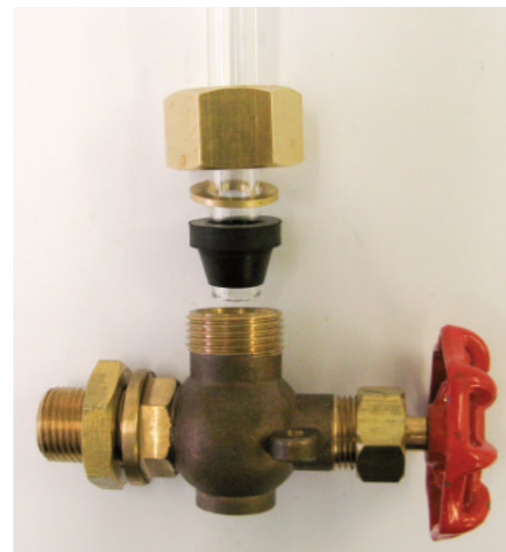
Detail showing the glass seal on a fig 61 Tank Gauge.
